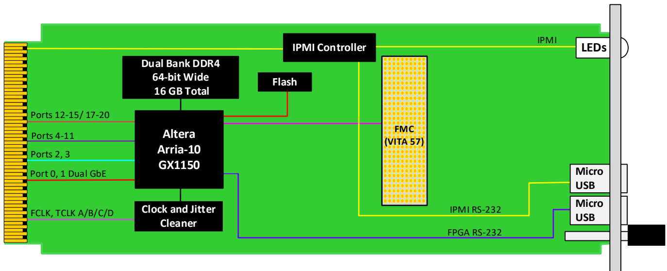
Figure 2: AMC536 Functional Block Diagram
